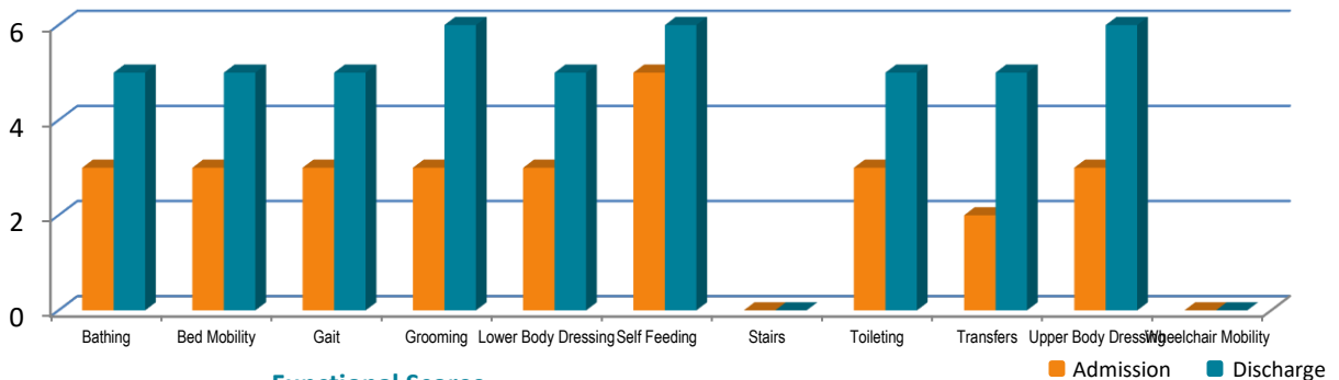
Functional Scores
